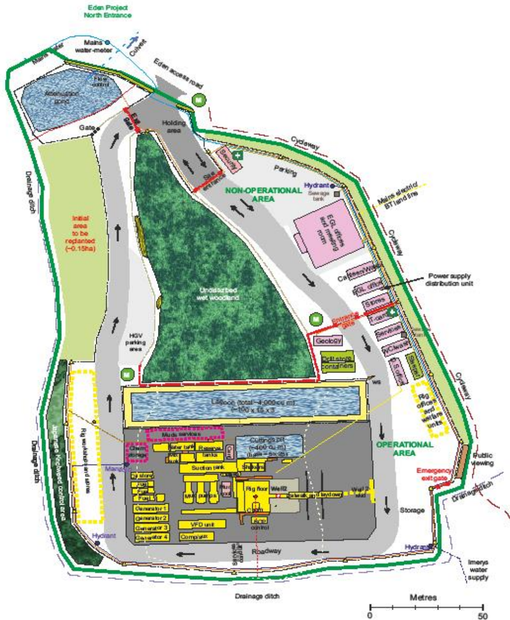
Proposed Layout of the Deep Geothermal Site at the Eden Project, Cornwall during the Construction Phase
