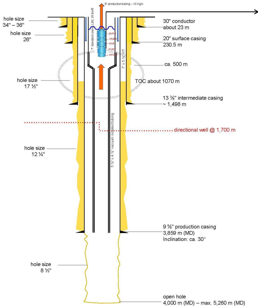
Schematic cross-section of Well EG-1 showing the coaxial installation
